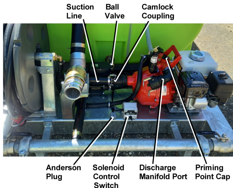
Figure 5 – Tank Filling Operation
