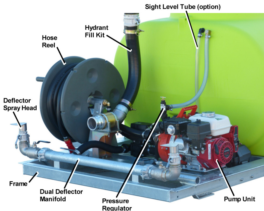
Figure 2 – Component Identification
