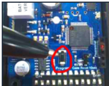
Figure 12 – SuperReel Remote Control Pairing
