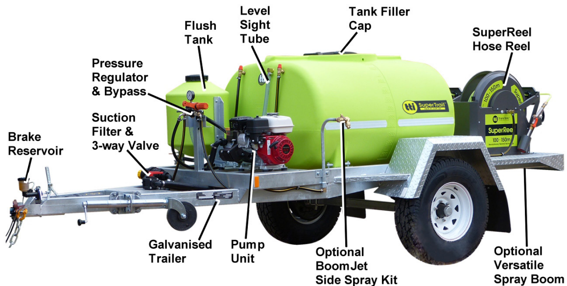
Figure 1 – Component Identification – SuperTrail with side-mounted BoomJet nozzle option
