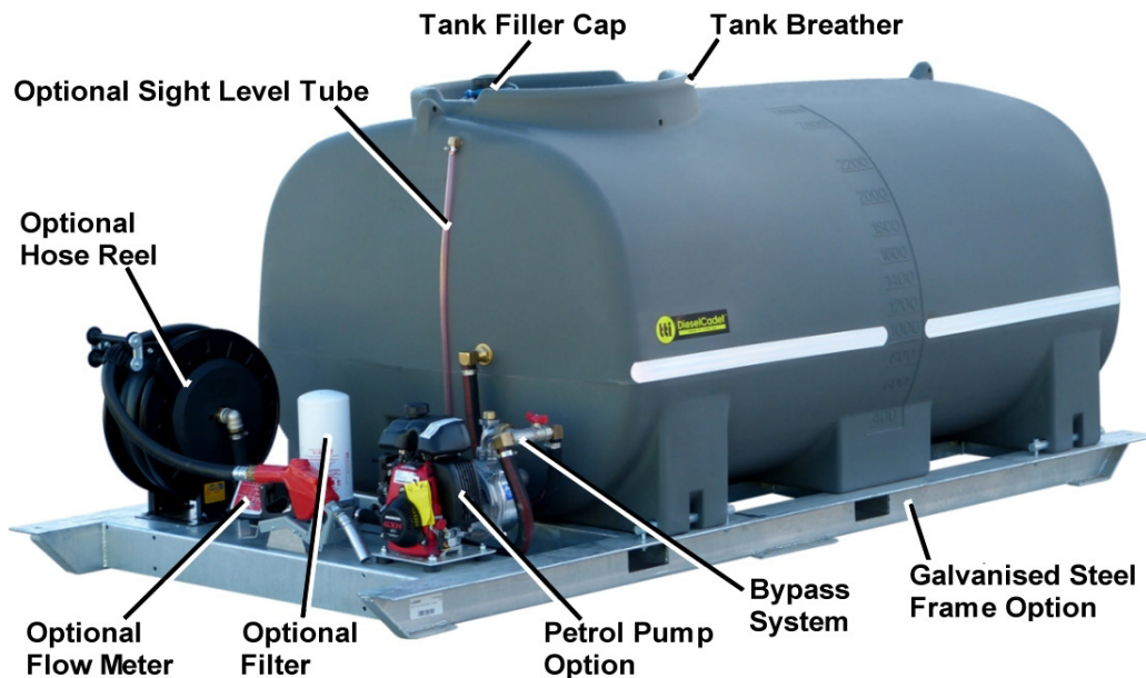
Figure 3 – Component Identification – DieselCadet with Frame and Petrol-powered Pump
