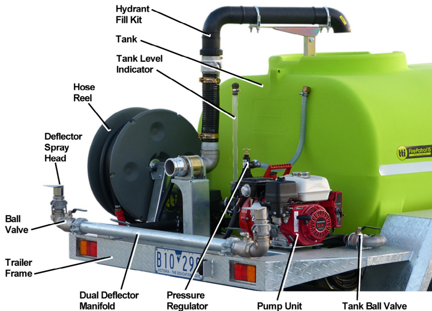
Figure 1 – Component Identification
