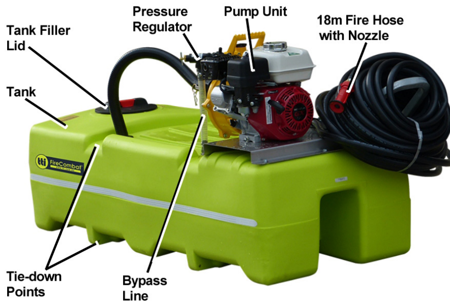
Figure 1 – Component Identification
